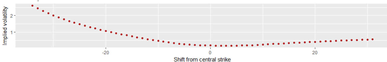
Figure 1. Volatility smile of the call RTS option on the 16th of November 2017
