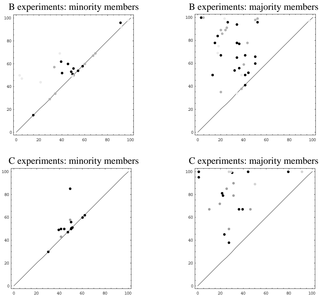
Figure 3b: Cutpoints
